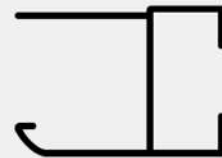
BI.FOLD DOOR INNER CENTRE JOINT (BFD-07)
