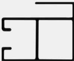
WINDOW INNER W/- HOCK (TIPIS)
