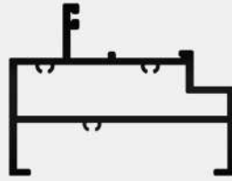
CASEMENT BIG OUTER (BIG-75)
