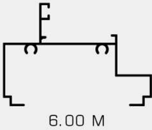
CASEMENT BIG OUTER (BIG-22)
