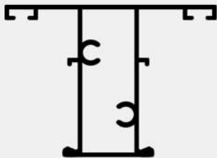
CASEMENT MULLION (BIG-75)
