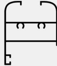
CASEMENT INNER W/O BEADING (BIG-75)
